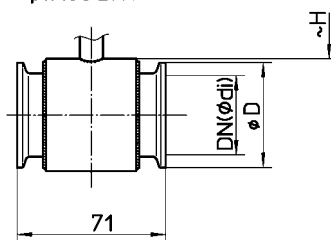
Clamping joint per DIN 32676, ISO 2852 and Tri-Clamp
